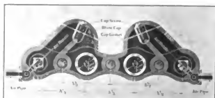
Fig. 3254. Valve of Leach Pneumatic Double Sander. American Locomotive Sander Co.
